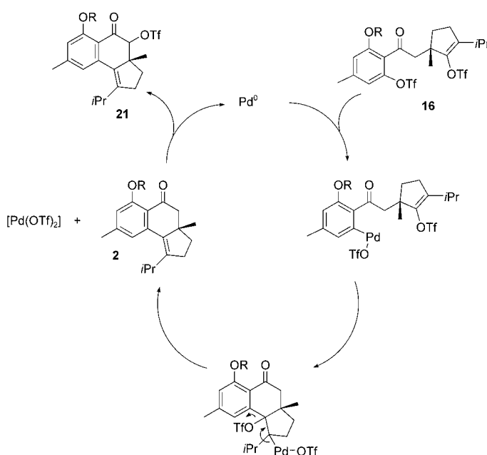
Figure 4. Proposed mechanism for the formation of 21 .
