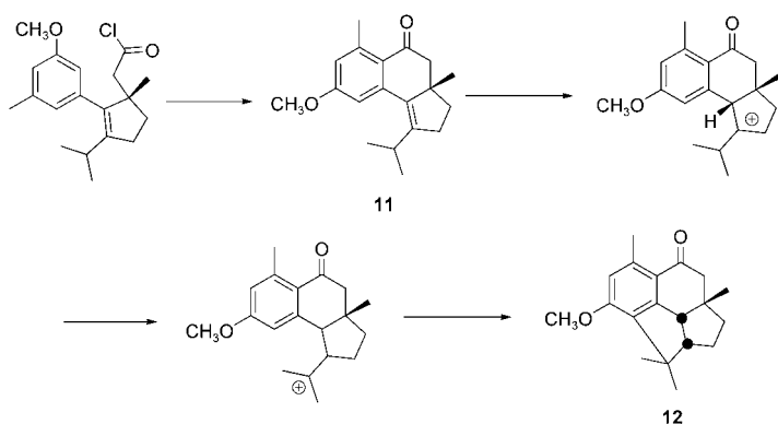
Scheme 3. Proposed mechanism for the formation of 12 .
