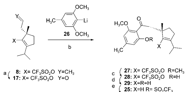
Scheme 8. Synthesis of substrate 25 for Heck reaction. a) cat. \text{OsO}_4 , NMO, \text{THF}/\text{H}_2\text{O} , then add \text{NaIO}_4 . b) i) DME, -55^{\circ}\text{C} . ii) Dess–Martin periodinane, \text{NaHCO}_3 , \text{CH}_2\text{Cl}_2 , rt, 75 % from 8 . c) \text{BCl}_3 , \text{CH}_2\text{Cl}_2 , -20^{\circ}\text{C} , 86 %. d) 10 mol % \text{Pd}(\text{OAc})_2 , 20 mol % dppf, \text{HCO}_2\text{H} , (\text{C}_2\text{H}_5)_3\text{N} , DMF, 70^{\circ}\text{C} , 1 h, 94 %. e) (\text{CF}_3\text{SO}_2)_2\text{O} , pyridine/ \text{CH}_2\text{Cl}_2 , 0^{\circ}\text{C} , 94 %.
