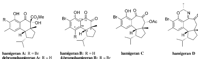
Figure 1. Structure of hamigerans.
