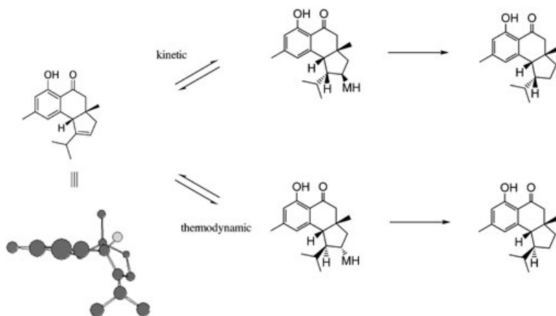
Scheme 10. Kinetic versus thermodynamic control of diastereoselectivity of hydrogenation.
