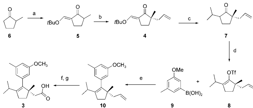
Scheme 2. Synthesis of carboxylic acid 3 . a) NaOMe, HCO 2 Et, PhH, 0°C to rt, then p TsOH, t BuOH, reflux, 61%. b) i) LDA, DME, –78°C to 0°C. ii) t BuOH, Me 3 SnCl, DME, 0°C. iii) 0.5 mol% [( \eta^3 -C 3 H 5 )PdCl] 2 , 1 mol% ( R,R )-ligand, allyl acetate, DME, –78°C to rt, 77%. c) LiCuMe 2 , Et 2 O, –20°C to rt, 89%. d) LDA, PhNTf 2 , THF, 87%. e) 2 equiv arylboronic acid 9 , 2.5 mol% [Pd(PPh 3 ) 4 ], KBr, K 3 PO 4 , dioxane, 85°C, 94%. f) 1.3 mol% OsO 4 , NMO, THF/H 2 O, 0°C to rt, then NaIO 4 , THF/H 2 O, 86%. g) Jones reagent, acetone, 75%.
