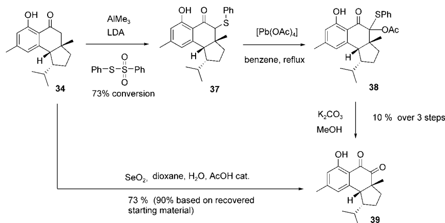
Scheme 11. Formation of diketone 39 .
