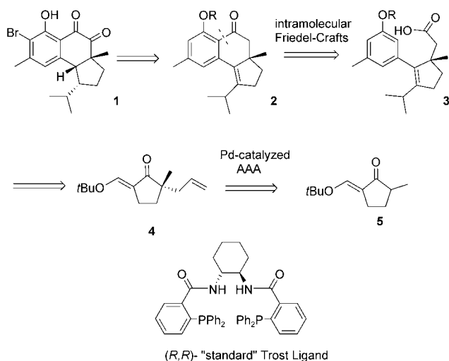
Scheme 1. Synthetic strategy envision for hamigeran B.
