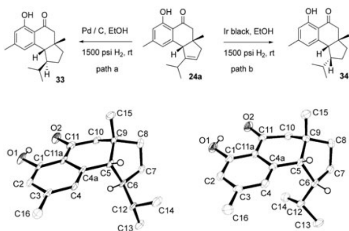
Scheme 9. Orthogonality between the thermodynamic and kinetic control in hydrogenation by choice of catalyst.
