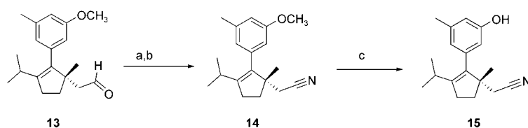
Scheme 4. Formation of nitrile 15 . a) \text{NH}_2\text{OH}\cdot\text{HCl} , \text{CH}_3\text{CO}_2\text{Na} , \text{CH}_3\text{CN}/\text{H}_2\text{O} , 1 h, rt, 98 %. b) [\text{RuCl}_2(p\text{-cymene})]_2 , MS 4 Å, \text{CH}_3\text{CN} , 80 °C, 15 min, 76 %. c) \text{BBr}_3 , \text{CH}_2\text{Cl}_2 , -78 °C to 0 °C, 85 %.
