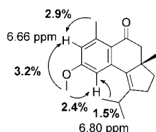
Figure 2. NOE correlations for 11 .
