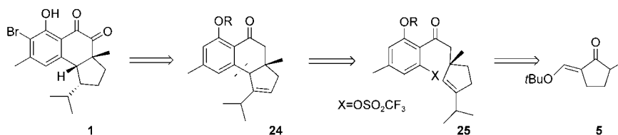
Scheme 7. Final retrosynthetic analysis.
