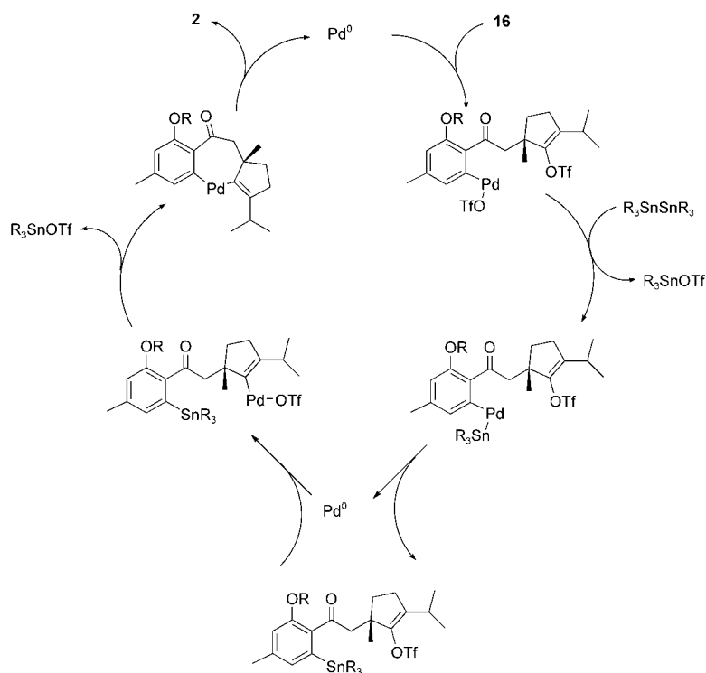
Figure 3. Aryl triflate/vinyl triflate coupling.
