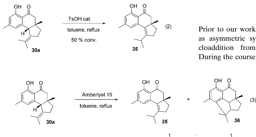
Scheme 10. Kinetic versus thermodynamic control of diastereoselectivity of hydrogenation.
