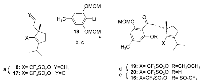
Scheme 6. Synthesis of substrate 16 . a) cat. \text{OsO}_4 , NMO, THF/ \text{H}_2\text{O} then \text{NaIO}_4 . b) \text{Et}_2\text{O} , -78 to 5 , 94%. c) Jones reagent, acetone, 78%. d) aq. \text{H}_2\text{SO}_4 , THF, 56%. e) (\text{CF}_3\text{SO}_2)_2\text{O} , pyridine/ \text{CH}_2\text{Cl}_2 , 95%.
